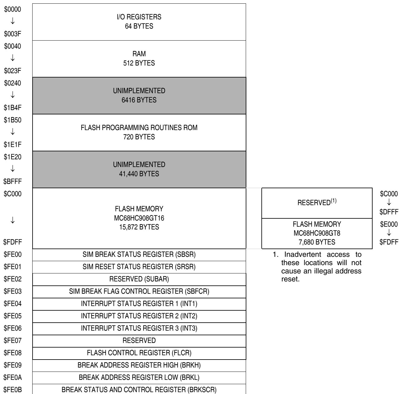
Figure 2-1. Memory Map
