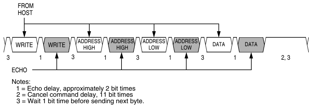
Figure 19-16. Write Transaction
