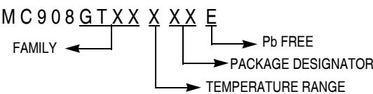
Figure 21-1. Device Numbering System
