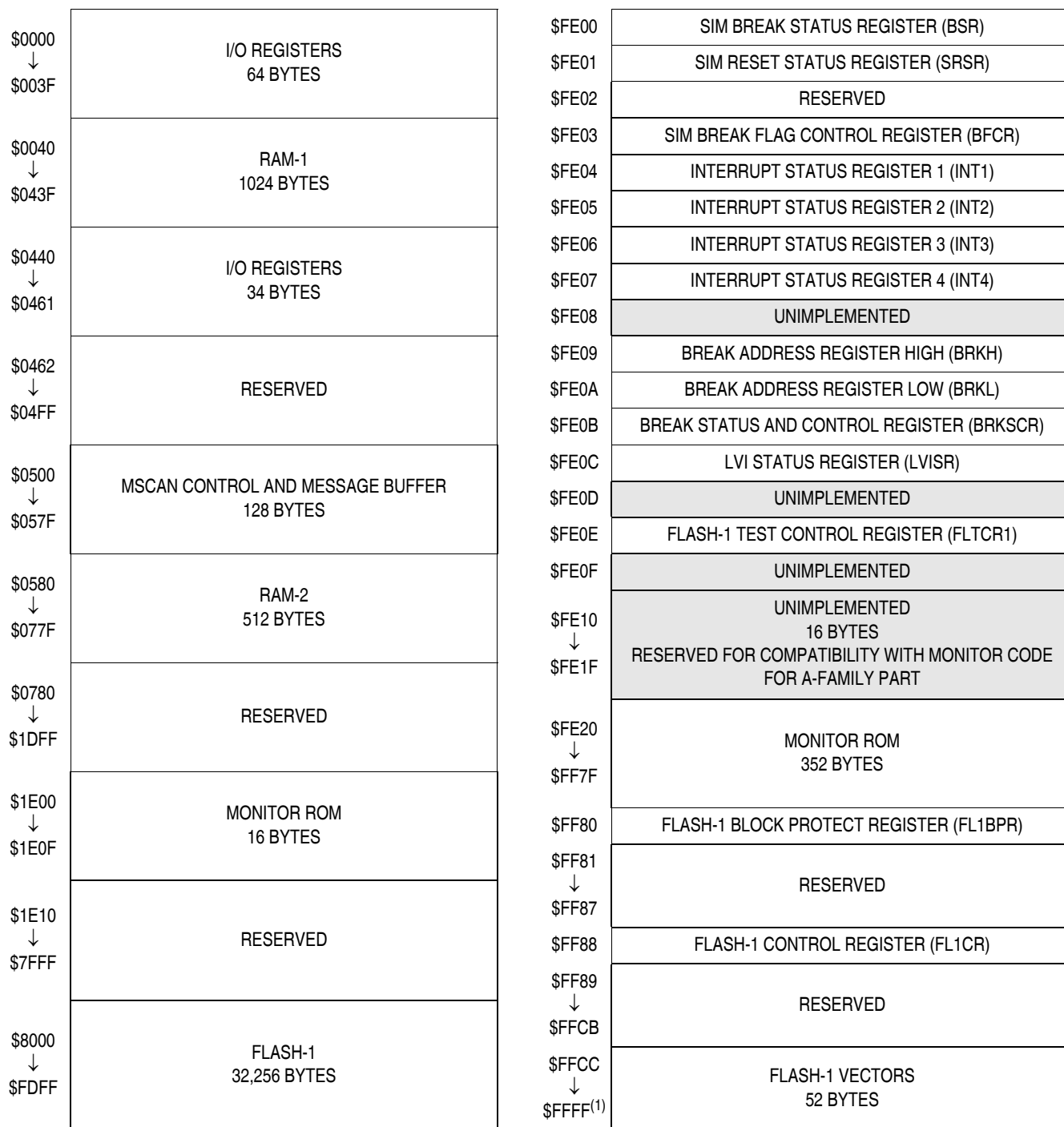
Figure B-2. MC68HC908GZ32 Memory Map
