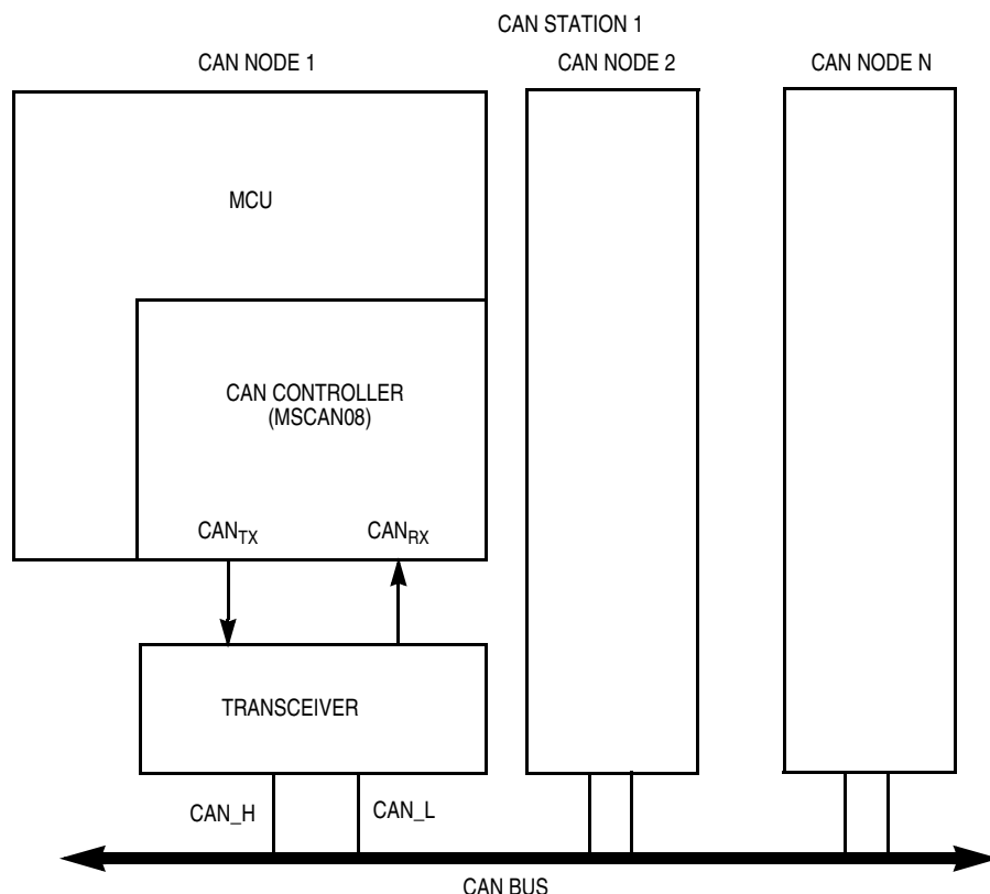
Figure 12-2. The CAN System
