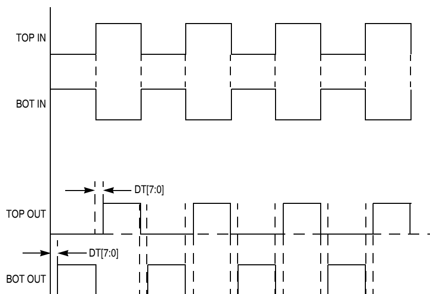
Figure 10-7. Deadtime Insertion Waveforms
