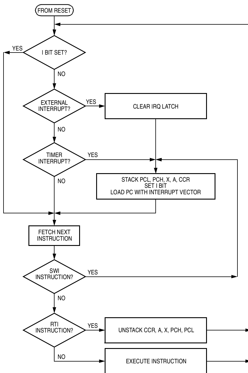
Figure 8-2. Interrupt Flowchart
