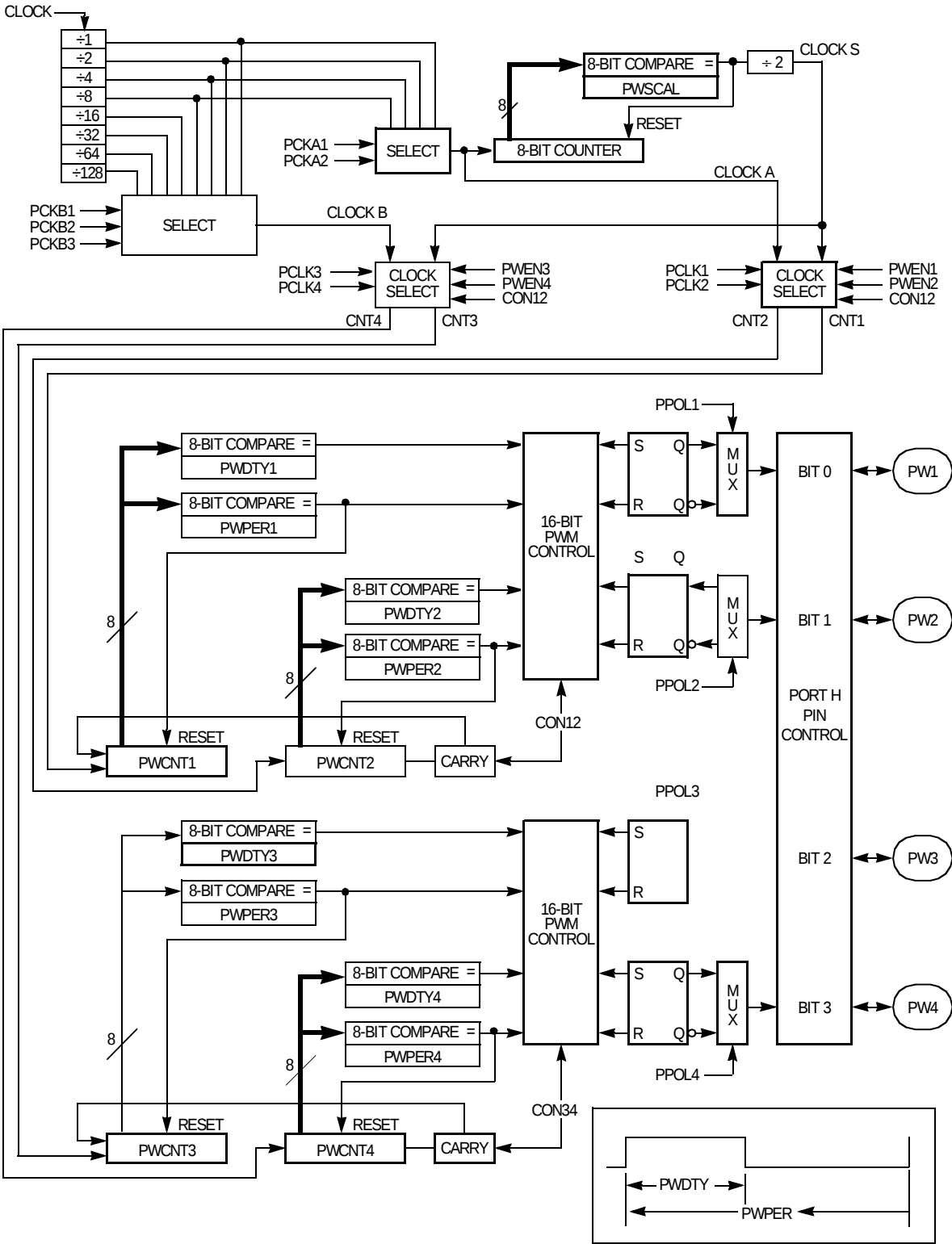
Figure 9-30. Pulse-Width Modulation Timer Block Diagram
