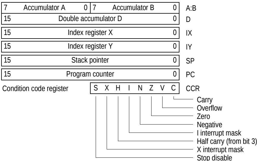
Figure 11-1. Programming model
