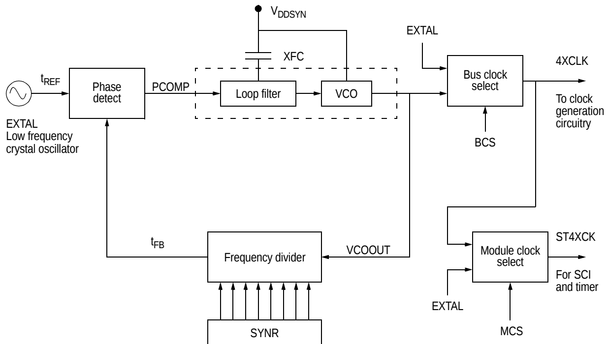
Figure 2-4. PLL circuit
