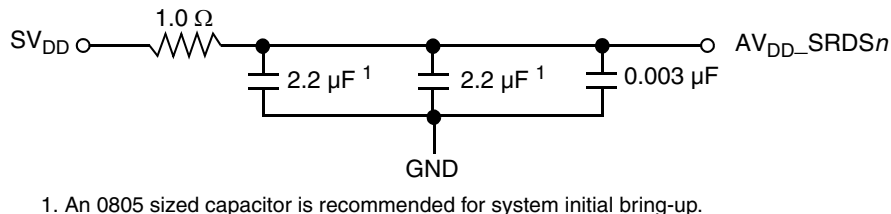
Figure 65. SerDes PLL Power Supply Filter
