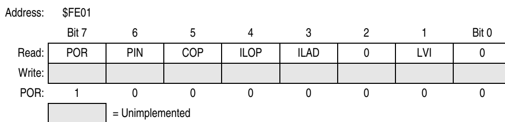
Figure 9-18. SIM Reset Status Register (SRSR)
