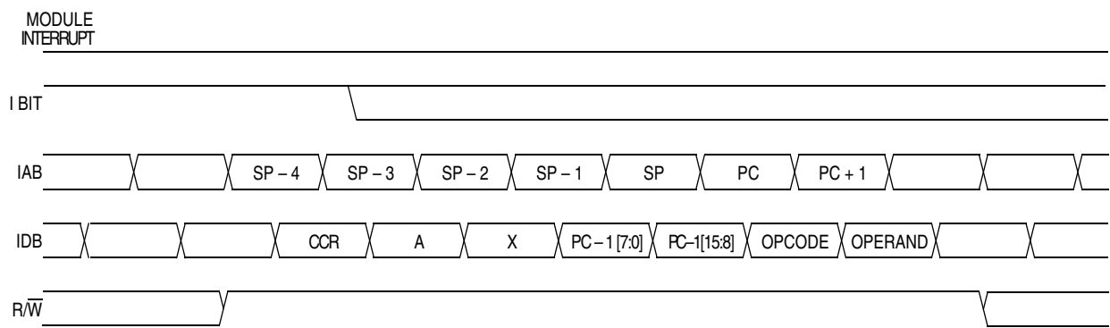
Figure 9-10. Interrupt Recovery
