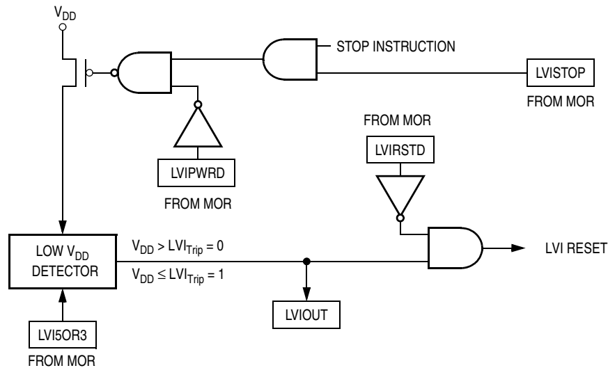
Figure 10-1. LVI Module Block Diagram
