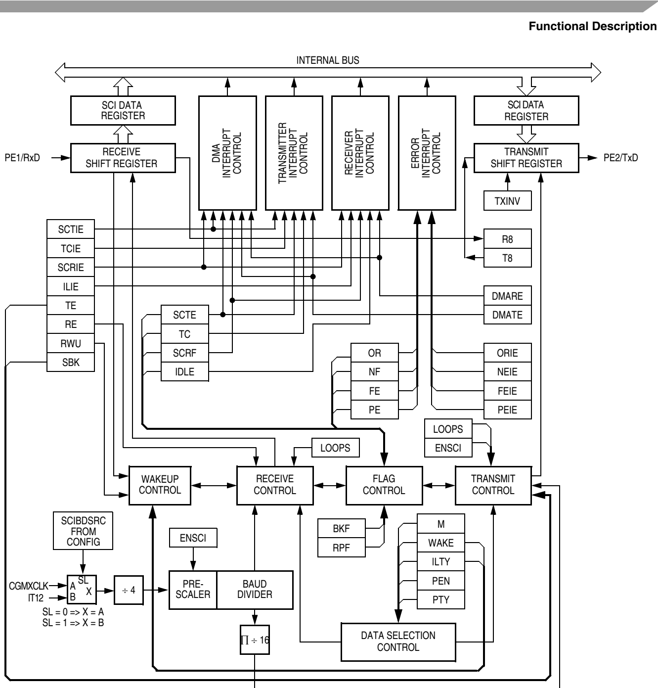
Figure 18-1. SCI Module Block Diagram
