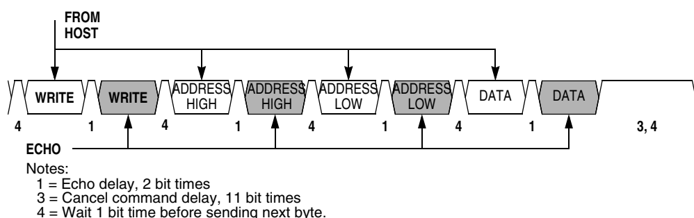
Figure 16-13. Write Transaction
