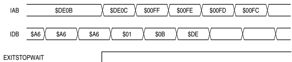
Figure 13-12. Wait Recovery from Interrupt
