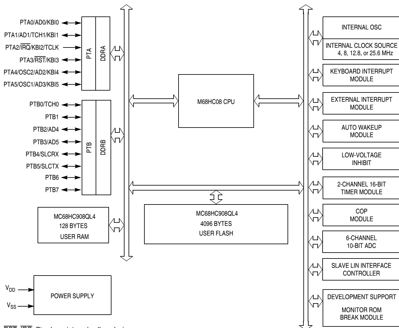
Figure 1-1. Block Diagram
