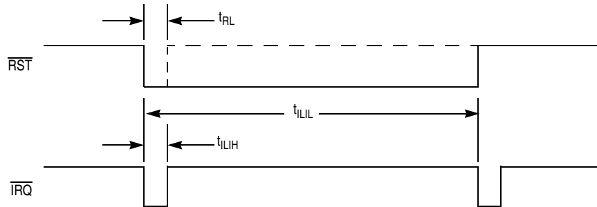
Figure 17-6. \overline{RST} and \overline{IRQ} Timing
