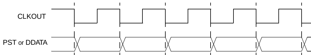
Figure 30-2. CLKOUT Timing
