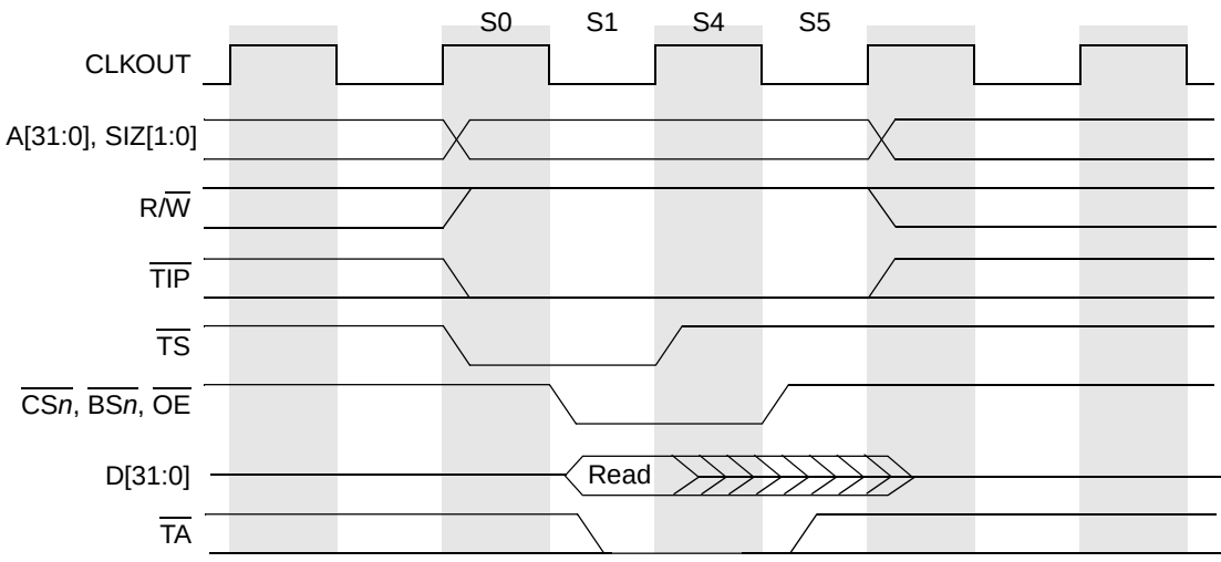
Figure 13-9. Read Cycle with Fast Termination
