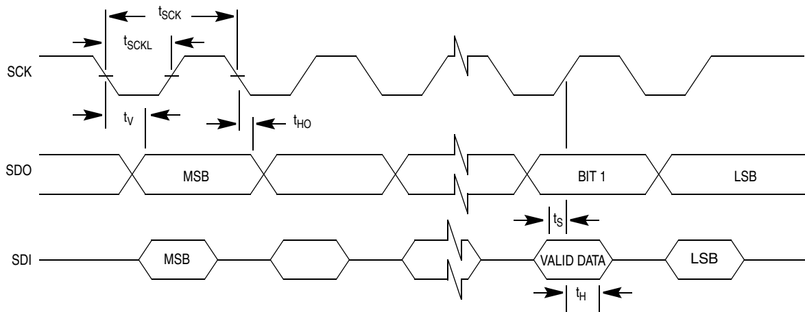
Figure 15-11. SIOPTiming Diagram
