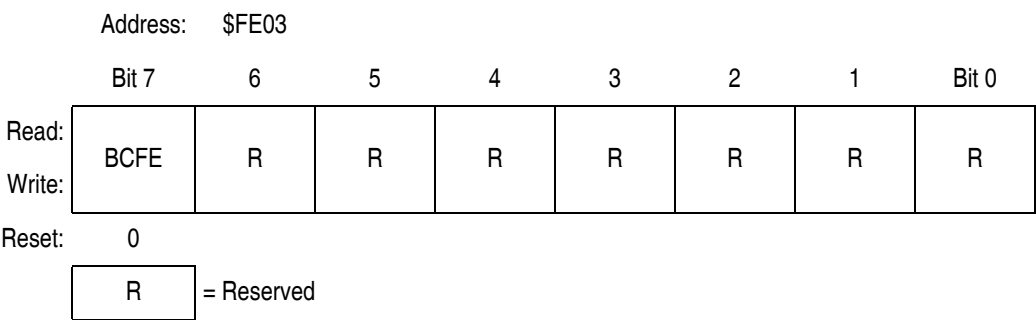
Figure 7-22. Break Flag Control Register (BFCR)
