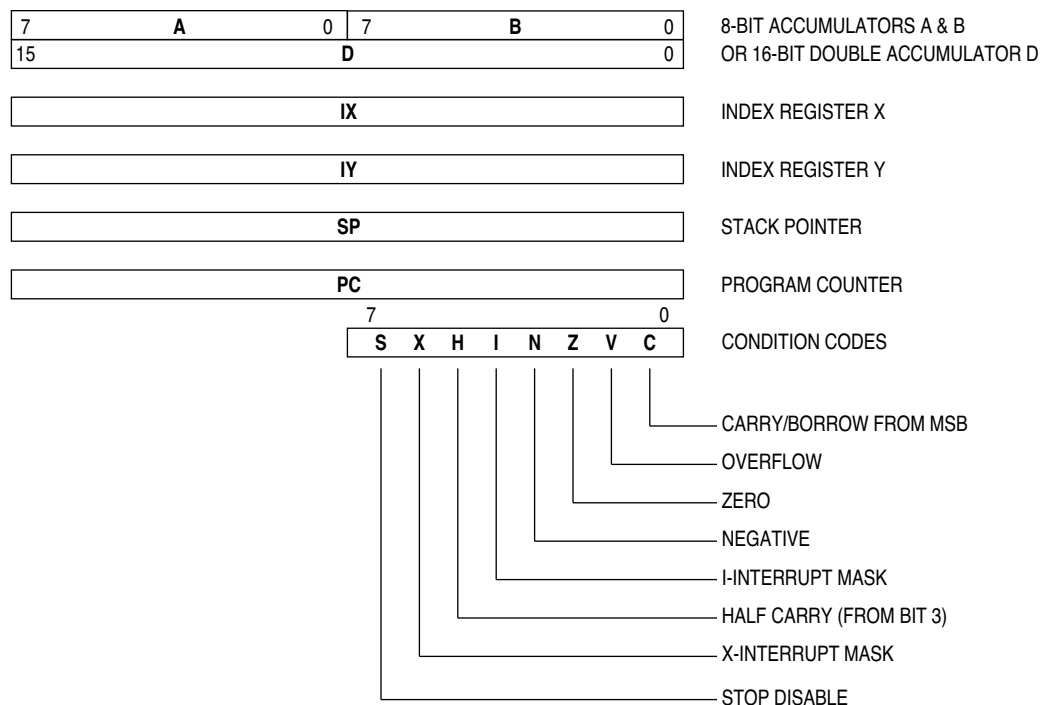
Figure 1-2 Programming Model
