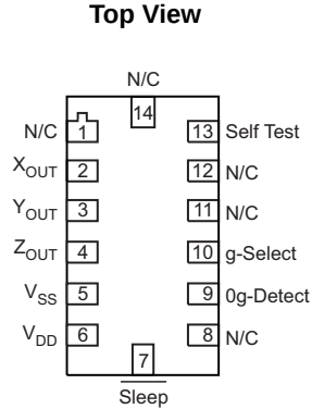
Figure 4. Pinout Description
