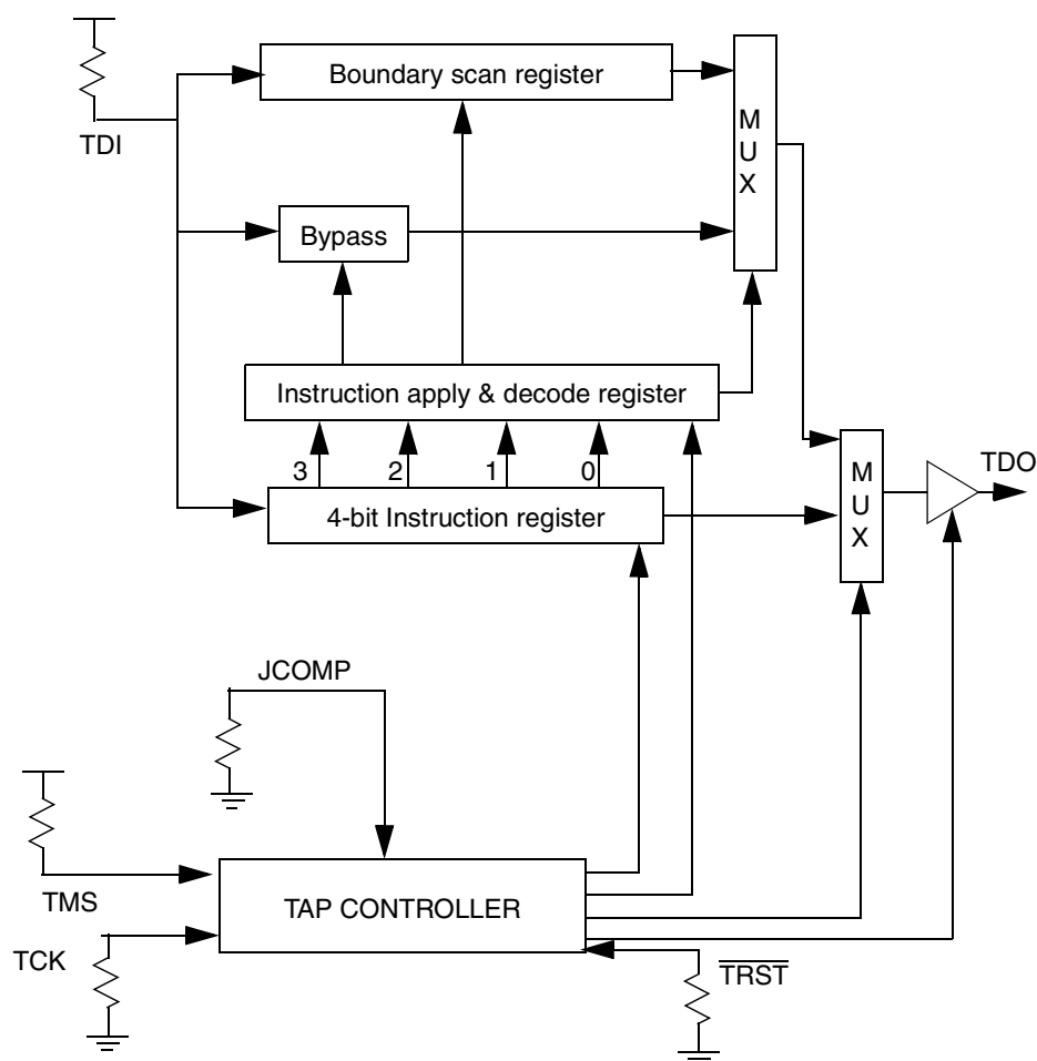
Figure 22-2 Test Logic Block Diagram
