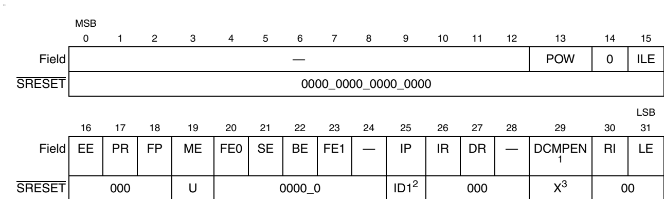
Figure 3-11. Machine State Register (MSR)
