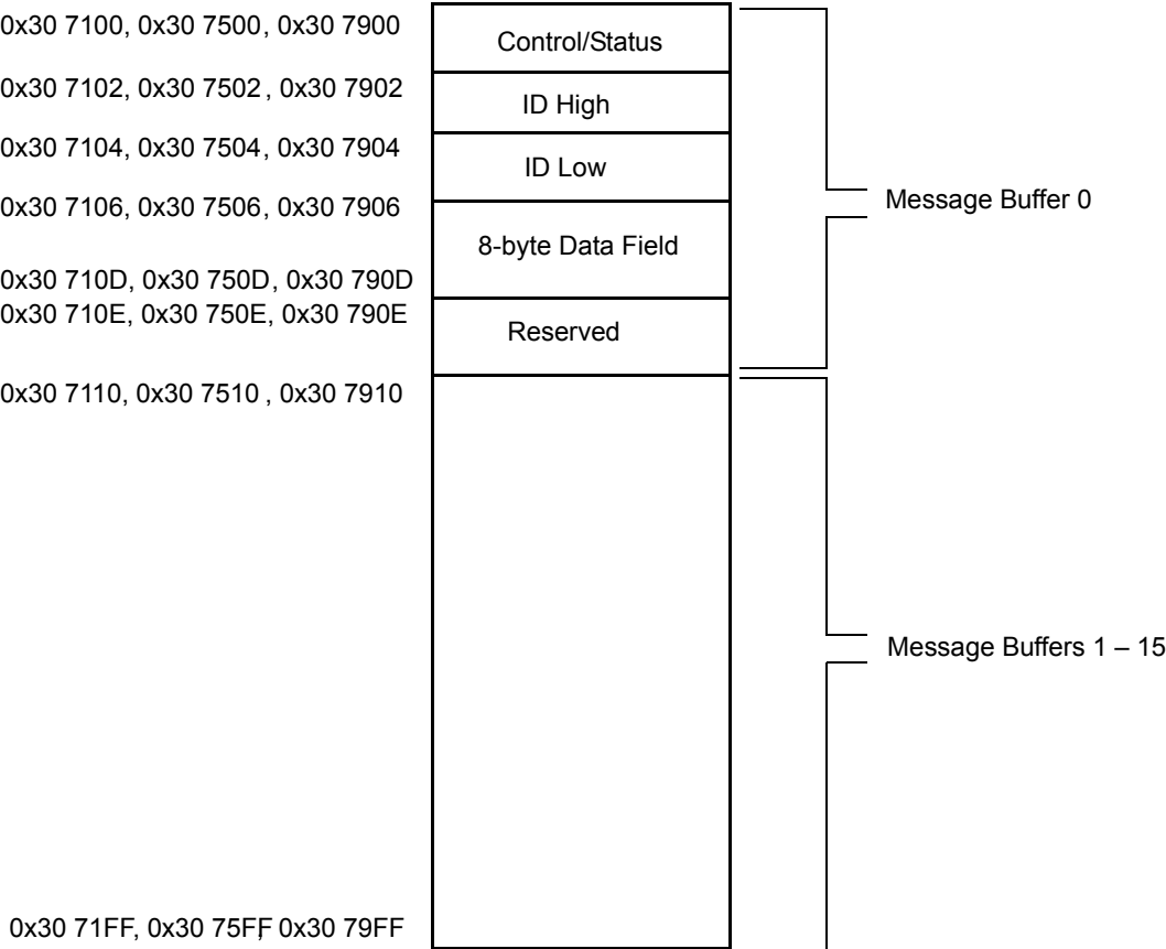
TouCAN Message Buffer Map Figure 16-8. TouCAN Message Buffer Memory Map
