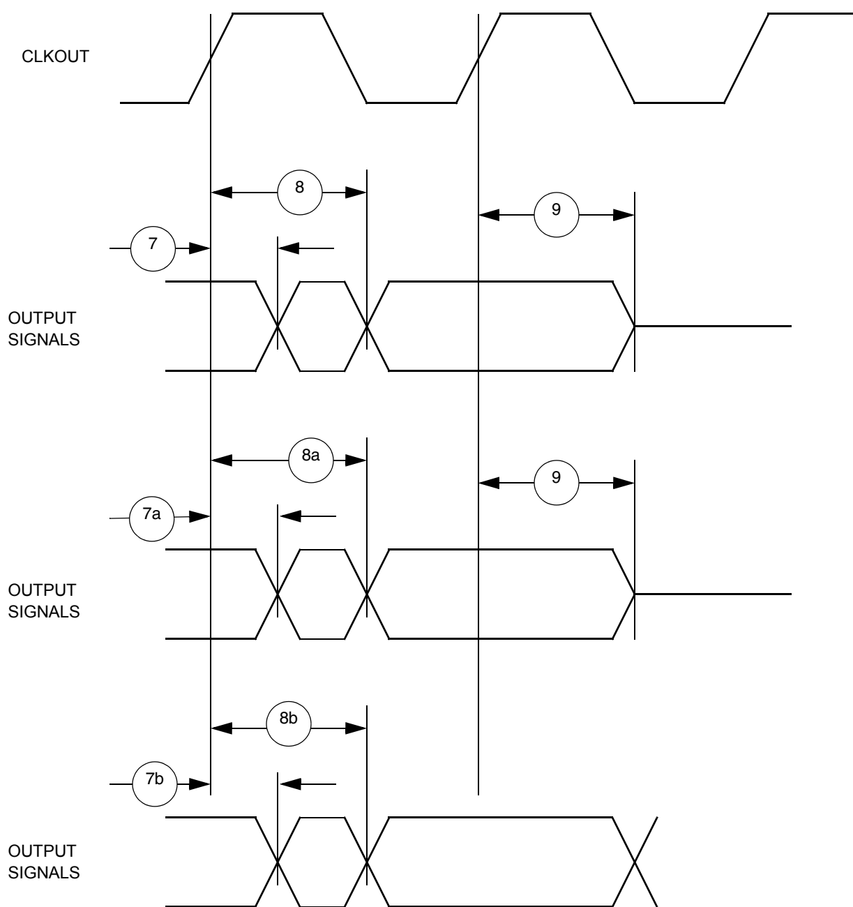
Figure F-11. Synchronous Output Signals Timing
