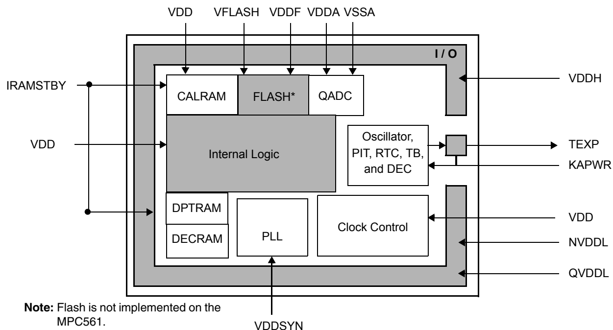
Figure 8-11. Basic Power Supply Configuration
