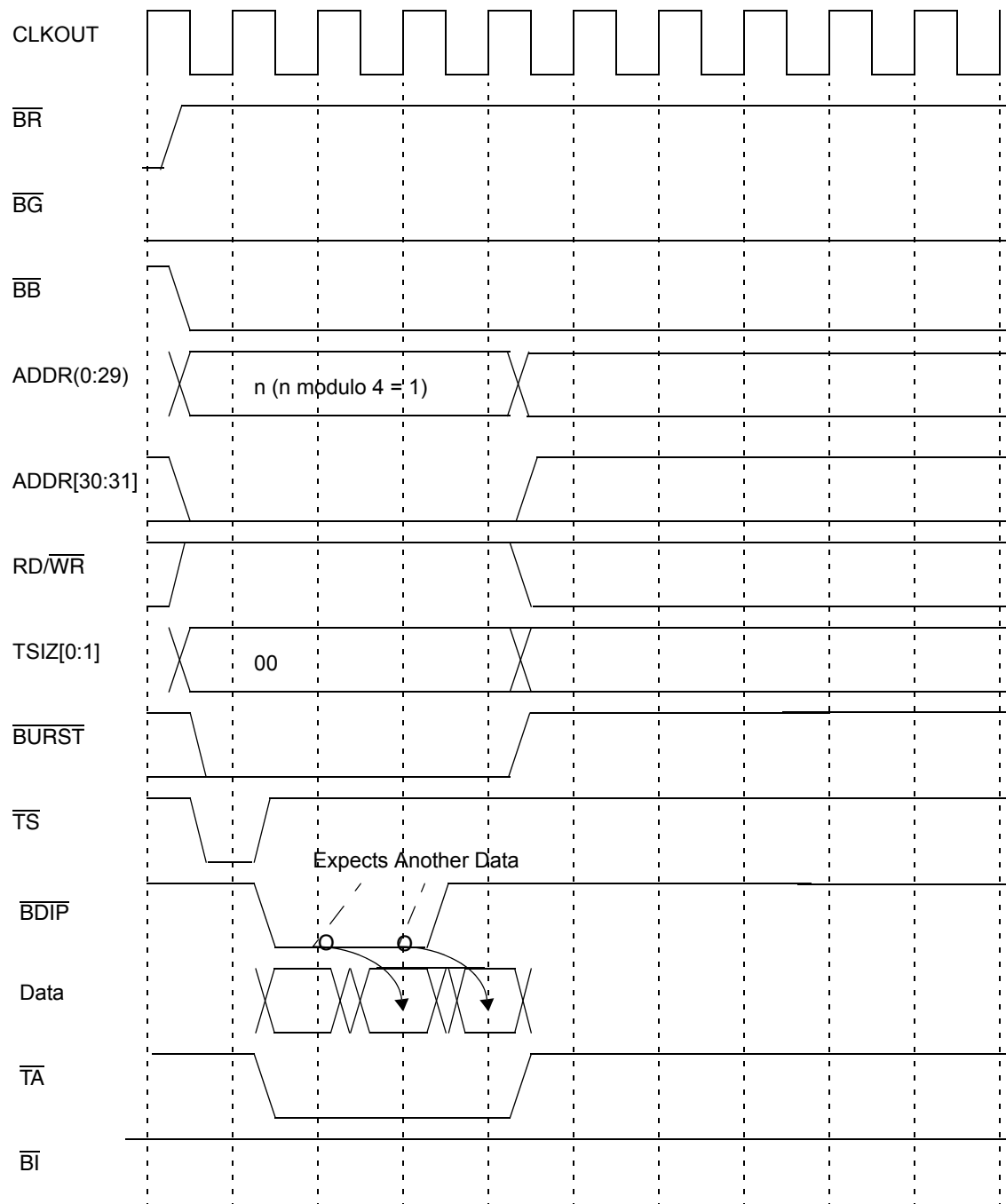
Figure 9-20. Non-Wrap Burst with Three Beats
