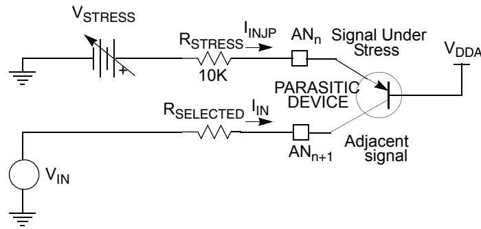
Figure 13-55. Input Signal Subjected to Positive Stress
