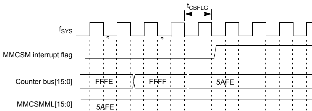
Figure G-54. MMCSM Counter Bus Reload to Interrupt Flag Setting Timing Diagram
