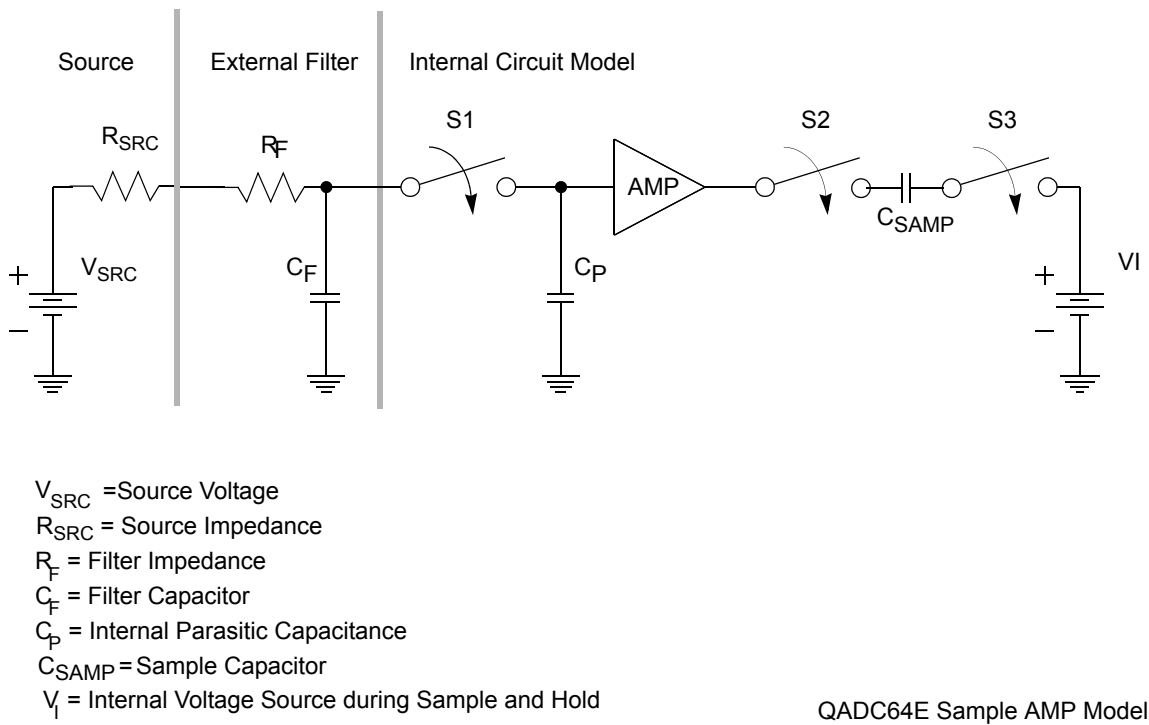
Figure 13-52. Electrical Model of an A/D Input Signal
