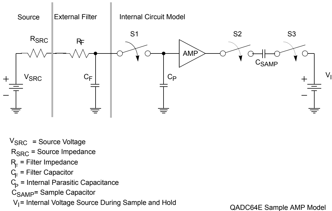
Figure 14-50. Electrical Model of an A/D Input Signal
