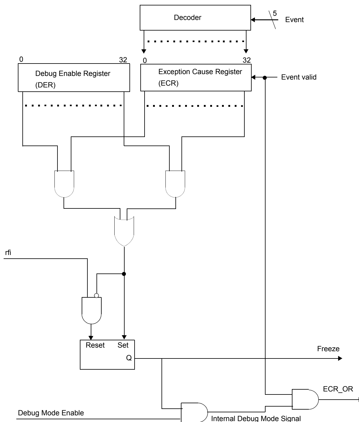
Figure 23-6. Debug Mode Logic
