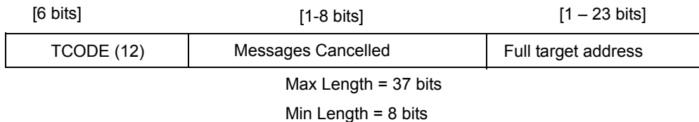
Figure 24-25. Direct Branch Synchronization Message Format (PTSM = 1)
