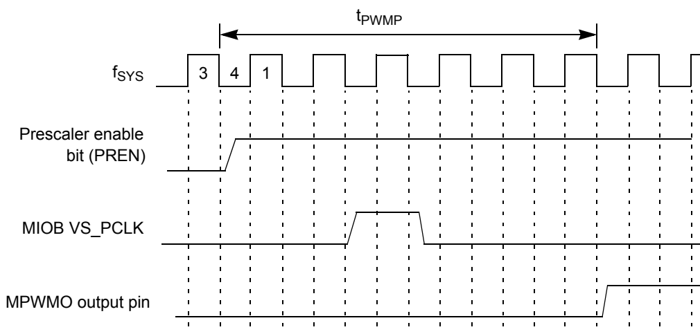
Figure G-48. MCPSPM Enable to MPWMO Output Pin Rising Edge Timing Diagram
