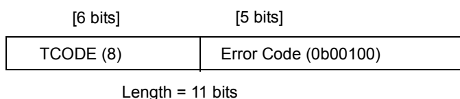
Figure 24-61. Error Message (Invalid Message) Format
