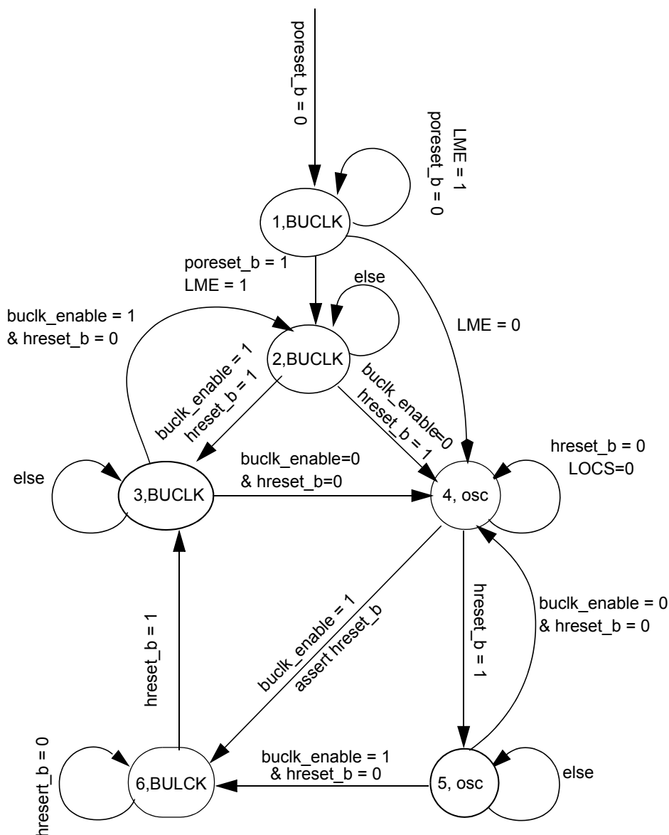
Figure 8-8. Clock Source Switching Flow Chart
