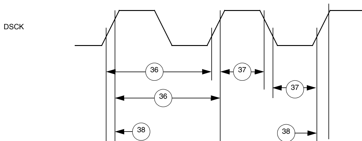
Figure G-27. Debug Port Clock Input Timing
