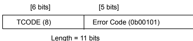
Figure 24-62. Error Message (Invalid Access Opcode) Format
