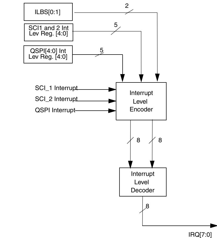
Figure 15-3. Interrupt Hardware Block Diagram
