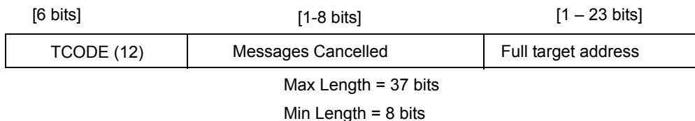
Figure 24-27. Indirect Branch Synchronization Message Format (PTSM = 1)
