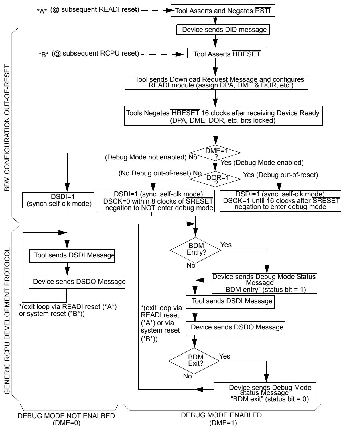
Figure 24-83. RCPU Development Access Flow Diagram
