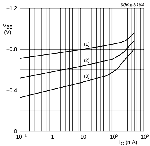
V_{CE} = -10\text{ V} (1) T_{amb} = -55^\circ\text{C} (2) T_{amb} = 25^\circ\text{C} (3) T_{amb} = 100^\circ\text{C}
