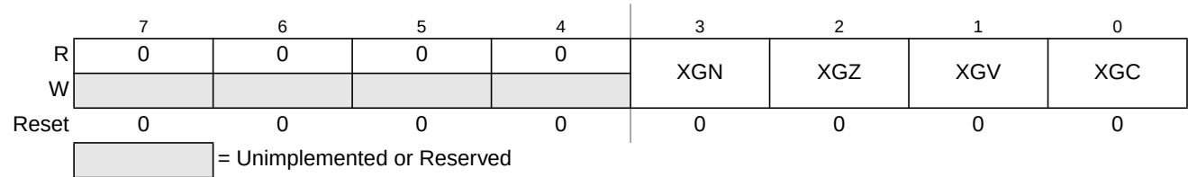
Figure 5-9. XGATE Condition Code Register (XGCCR)
