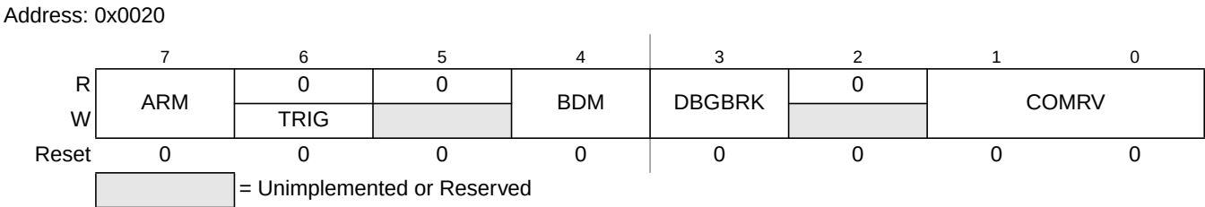
Figure 6-3. Debug Control Register (DBG1)
