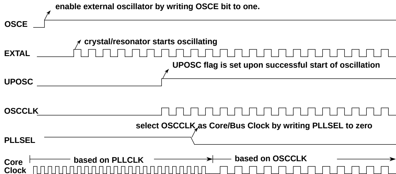
Figure 7-34. Enabling the External Oscillator
