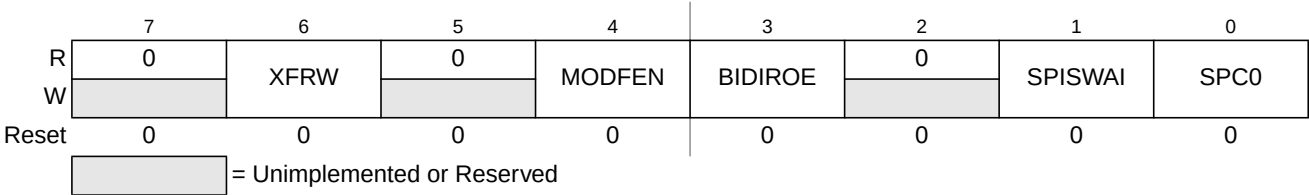
Figure 12-4. SPI Control Register 2 (SPICR2)
