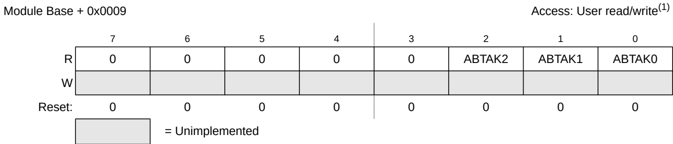
Figure 8-13. MSCAN Transmitter Message Abort Acknowledge Register (CANTAABK)
