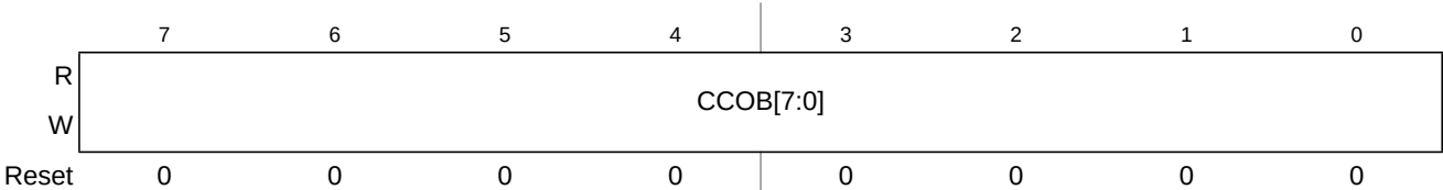
Figure 13-17. Flash Common Command Object Low Register (FCCOBLO)
