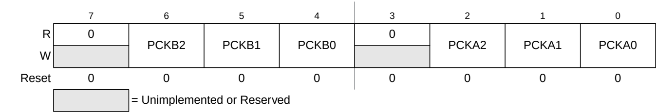
Figure 10-6. PWM Prescaler Clock Select Register (PWMPRCLK)
