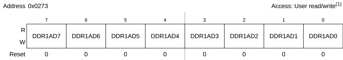
Figure 2-58. Port AD Data Direction Register (DDR1AD)
