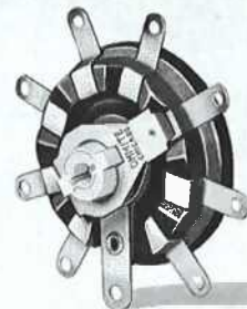
Fig. 215 - A Non-Shorting Type Switch (T-508).
