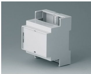
B6703106 RAILTEC C, 4 modules, Vers. IV PC (UL 94 V-0) light gray 2.80"x3.54"x2.28"
