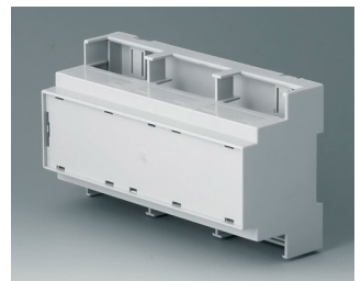
B6706106 RAILTEC C, 9 modules, Vers. IV PC (UL 94 V-0) light gray 6.30"x3.54"x2.28"
