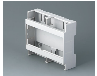
B6705800 RAILTEC C, 6 modules, flat, Vers. I PC (UL 94 V-0) light gray 4.18"x3.54"x1.26"
