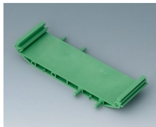
B6720441 RAILTEC SUP. 107, intermediate part PA 6 (UL 94 V-0) green 4.65"x1.38"x0.69"
