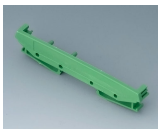
B6720445 RAILTEC SUP. 107, end section with foot PA 6 (UL 94 V-0) green 4.65"x0.45"x1.08"
