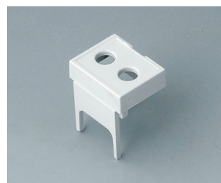
B6800114 Terminal guards, with holes, 7.5 mm & 7.62 mm PC (UL 94 V-0) light gray
