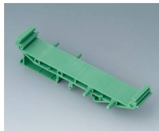
B6720442 RAILTEC SUP. 107, intermediate p. + foot PA 6 (UL 94 V-0) green 4.65"x0.73"x1.08"
