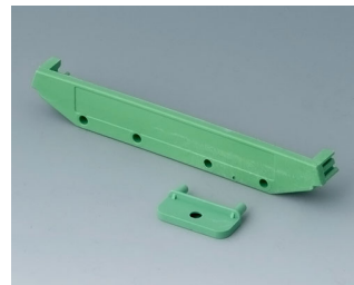
B6820542 Wall suspension element for SUP. 107 PA 6 (UL 94 V-0) green
