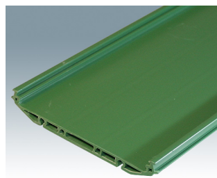
CIME/E/BExxx RAILTEC SUP. EXT 107, base section PA (UL 94 V-0) green 4.61"x0.71"
