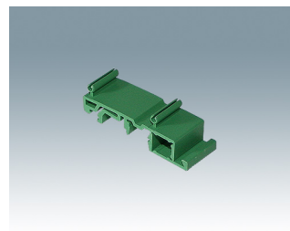
CIME/M/FE RAILTEC SUP. EXT 72, DIN rail foot PA (UL 94 V-0) green 0.79"x0.49"x2.36"
