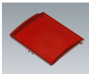
B6802301 Front lid convex without hinge PC (UL 94 V-0) red transparent
