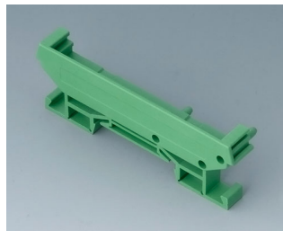
B6720335 RAILTEC SUP. 72, end section with foot PA 6 (UL 94 V-0) green 3.23"x0.44"x0.89"
