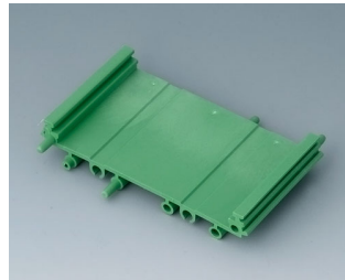
B6720332 RAILTEC SUP. 72, intermediate part PA 6 (UL 94 V-0) green 3.23"x1.77"x0.63"
