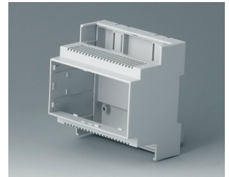
B6704102 RAILTEC C, 5 modules, Vers. II PC (UL 94 V-0) light gray 3.46"x3.54"x2.28"
