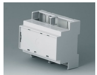
B6705106 RAILTEC C, 6 modules, Vers. IV PC (UL 94 V-0) light gray 4.17"x3.54"x2.28"
