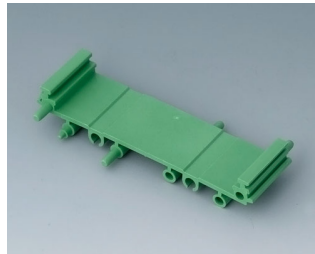
B6720331 RAILTEC SUP. 72, intermediate part PA 6 (UL 94 V-0) green 3.23"x0.89"x0.63"
