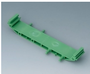
B6720440 RAILTEC SUP. 107, intermediate part PA 6 (UL 94 V-0) green 4.65"x0.73"x0.69"
