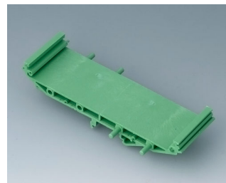
B6720443 RAILTEC SUP. 107, intermediate p. + foot PA 6 (UL 94 V-0) green 4.65"x1.38"x1.08"
