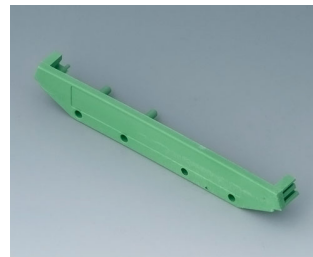
B6720444 RAILTEC SUP. 107, end section PA 6 (UL 94 V-0) green 4.65"x0.45"x0.69"
