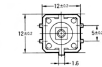
PCB Mounting (Top View) (Single-sided PCB, t=1.6 )
