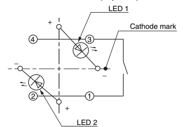
Terminal Arrangement/ Internal Connections (Top View)
