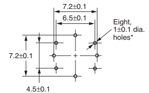
PCB Mounting (Top View)
