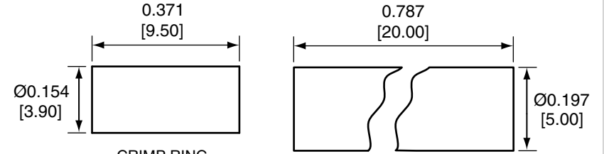
CRIMP RING
