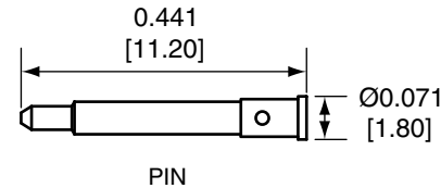
PIN
