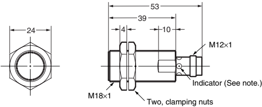
E2A-M18KS08-M1-□□/E2A-S18KS08-M1-□
