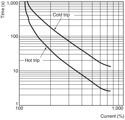
Overload Class 20
