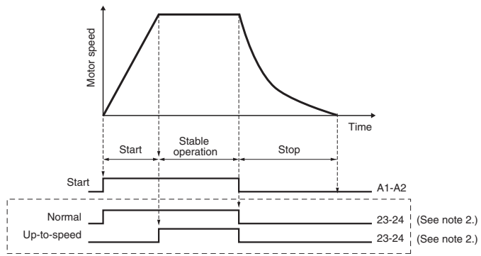
Operation Chart: Two-wire Connections with Forward/Reverse Rotation
