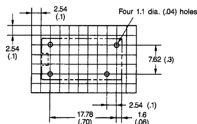
PC board dimensions (Bottom view)
