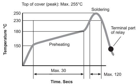
Recommended IRS Conditions (G6H-2F)
