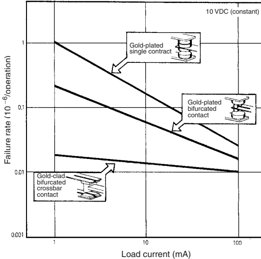
Failure Rate vs. Load Current
