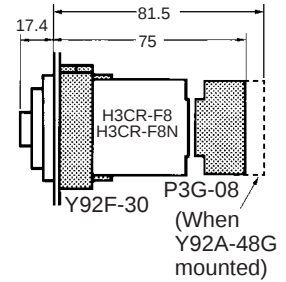
Dimensions with Back Connecting Socket P3G-08/P3GA-11
