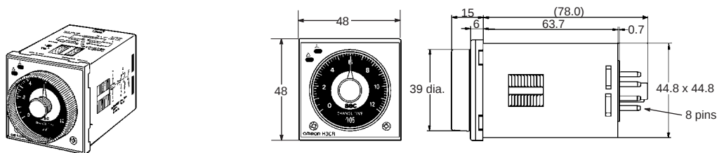
Dimensions with Set Ring
