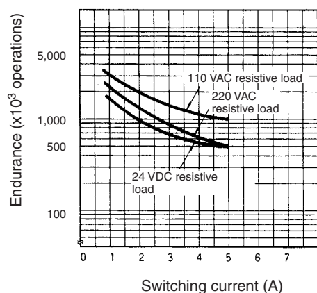
MY4-02, MY4F (Resistive Loads)
