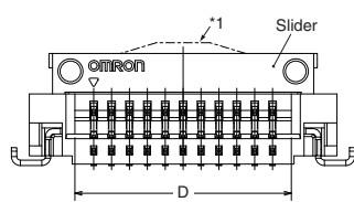
FPC insertion dimension
