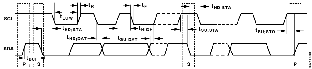
Figure 2. Diagram for Serial Bus Timing
