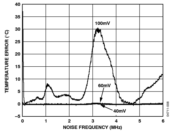
Figure 8. Remote Temperature Error vs. Common-Mode Noise Frequency
