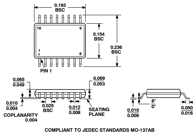
Figure 46. 16-Lead Shrink Small Outline Package [QSOP] (RQ-16)
