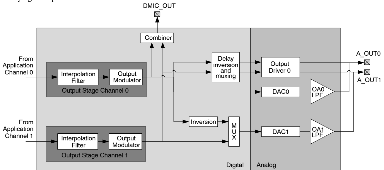
Figure 8. Output Stage
