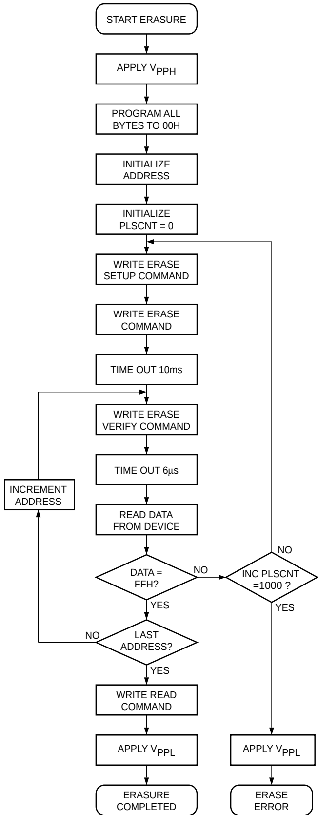
Figure 5. Chip Erase Algorithm (1)
