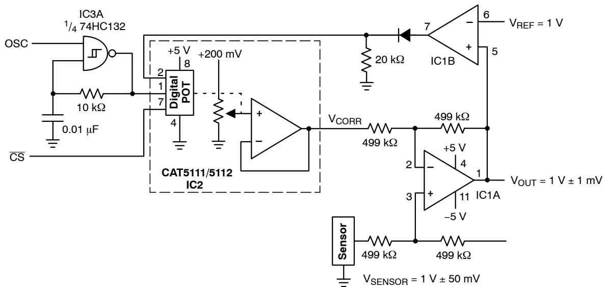
Figure 6. Programmable Instrumentation Amplifier
