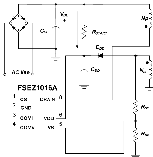
Figure 28. Startup Circuit
