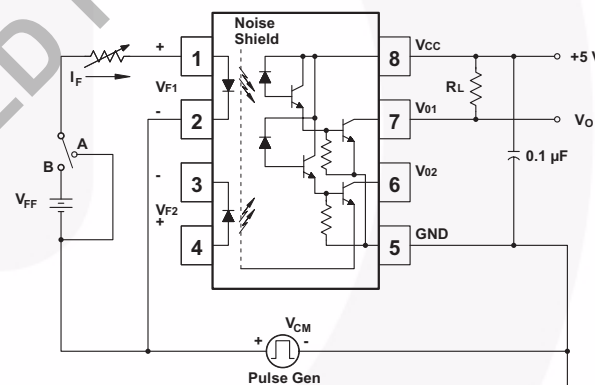
Test Circuit for HCPL2730 and HCPL2731
