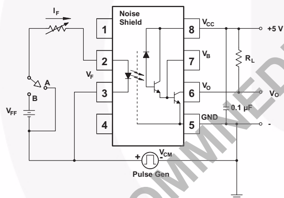
Test Circuit for 6N138 and 6N139
