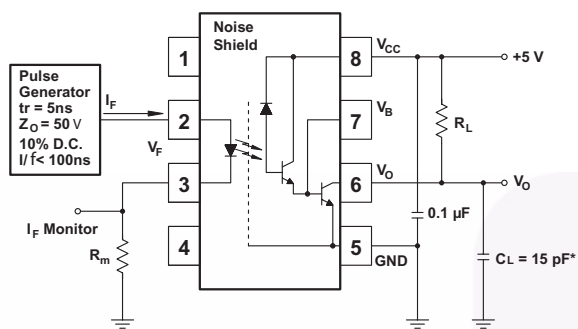
Test Circuit for 6N138, 6N139
