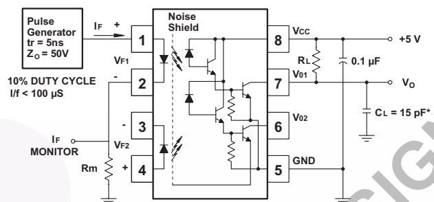
Test Circuit for HCPL2730 and HCPL2731
