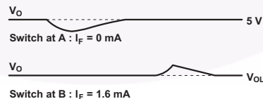
Fig. 25 Common Mode Immunity Test Circuit
