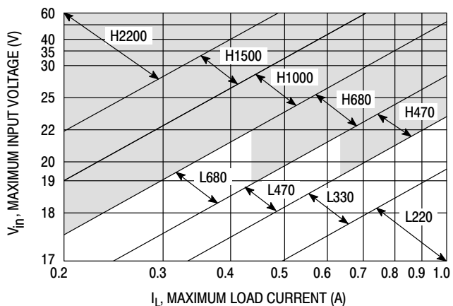
Figure 20. LM2575-15
