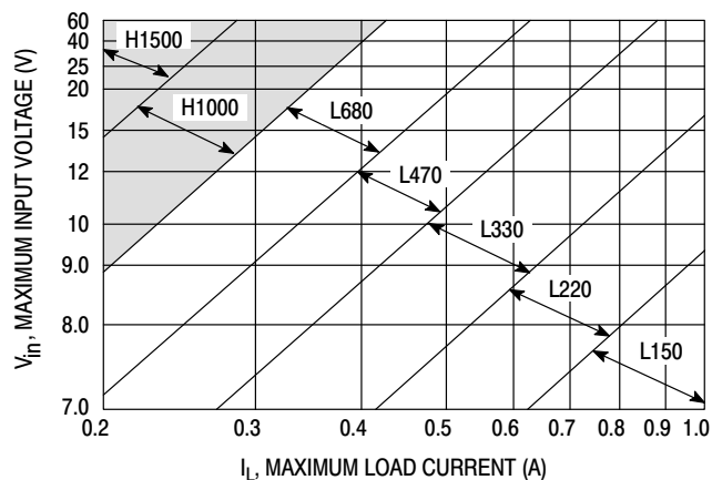
Figure 18. LM2575-5.0
