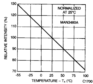
Fig. 3. Relative Luminous Intensity vs. Temperature
