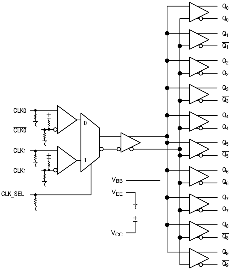
Figure 3. Logic Diagram
