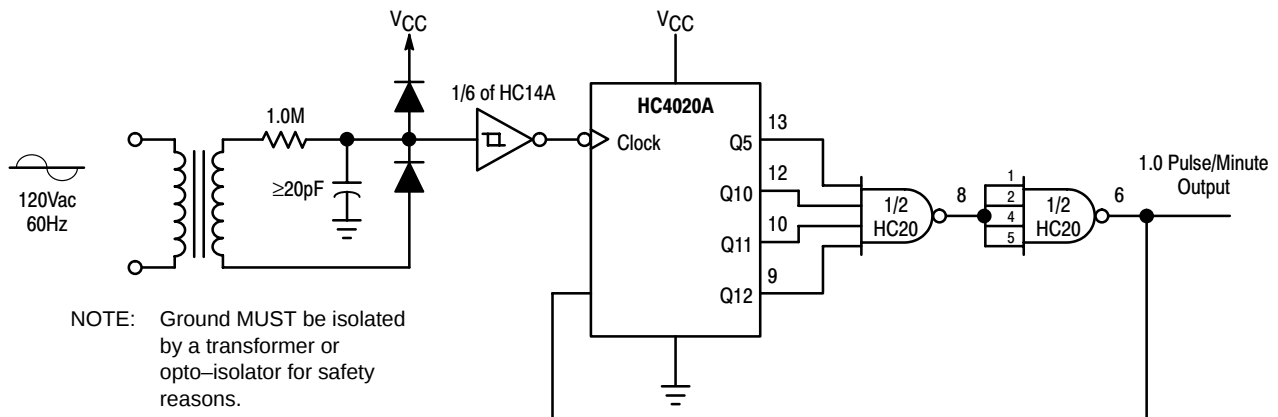
Figure 7. Time-Base Generator
