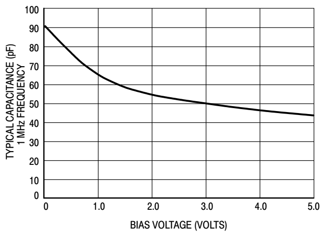
Figure 11. Capacitance
